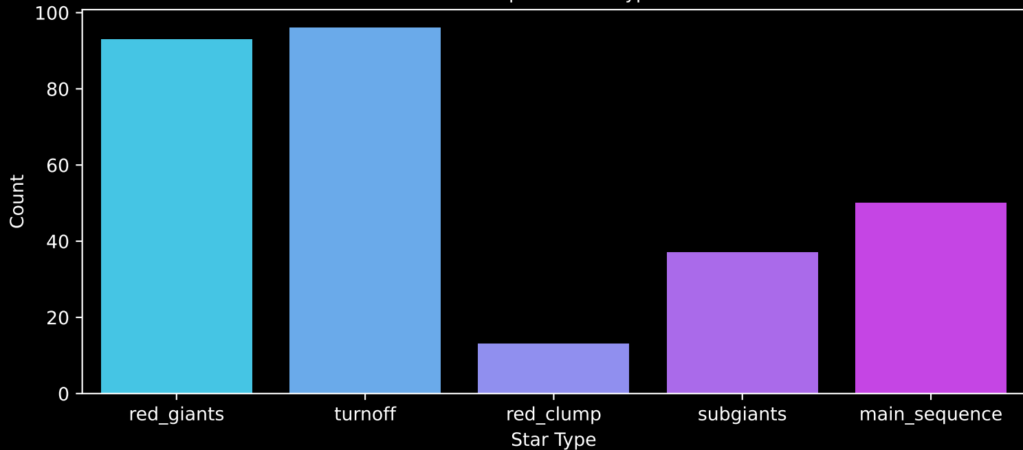
GALAH DR4 Field: [9404] Count plot of Star Type
