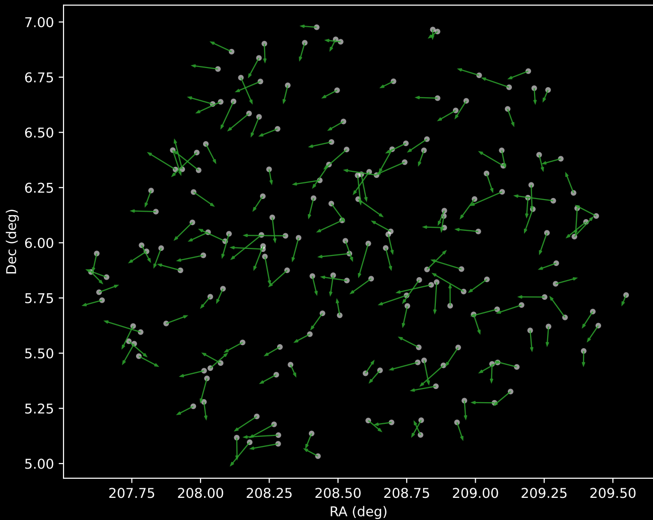
GALAH DR4 Cluster 4 Proper Motion Vectors (n=183)
