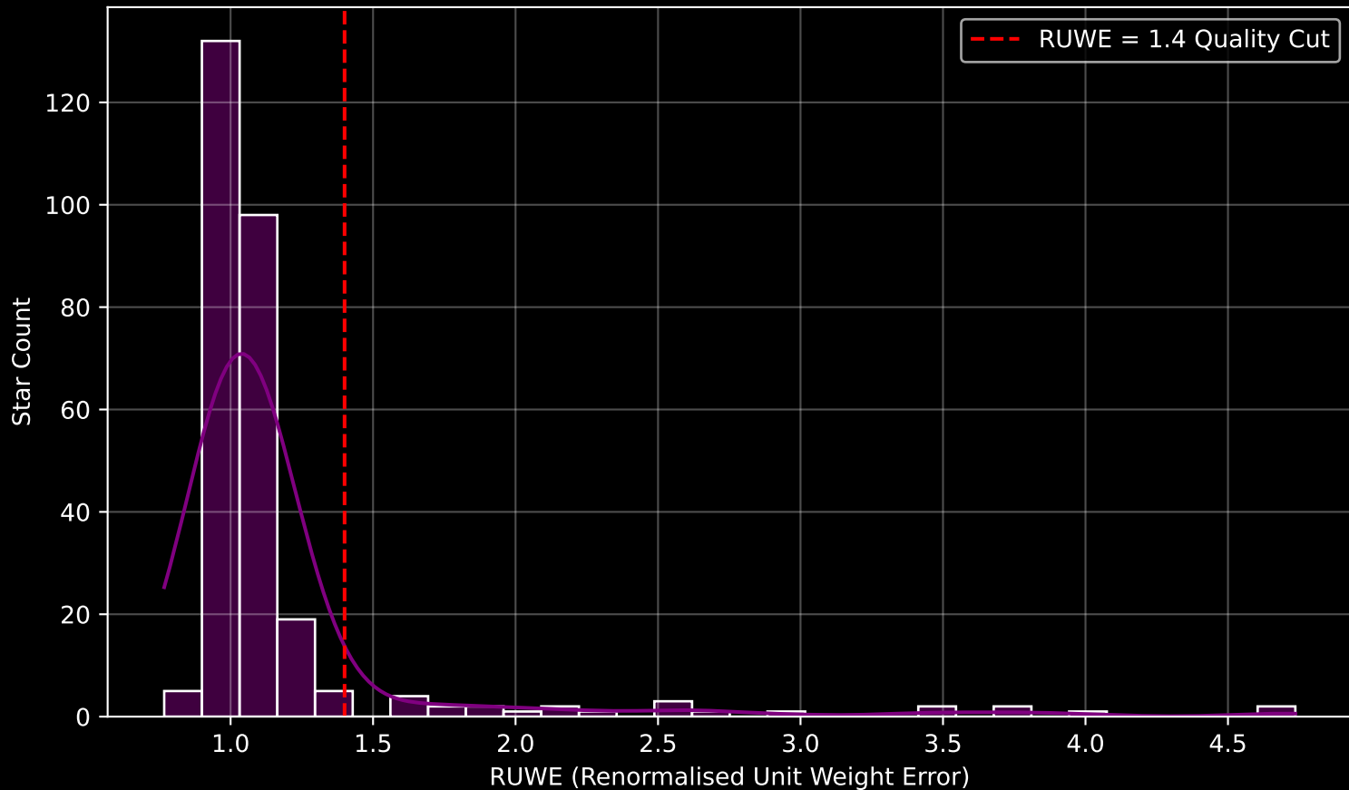
GALAH DR4 Field [9404] RUWE Distribution (n= 283)
